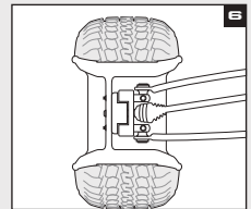
Reassemble tie rod, ball joints, brake caliper, axle nut, tire & wheel.
