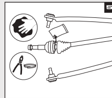
Empty the bag of grease into the CV joint/boot, clean sealing points & install clamps.
